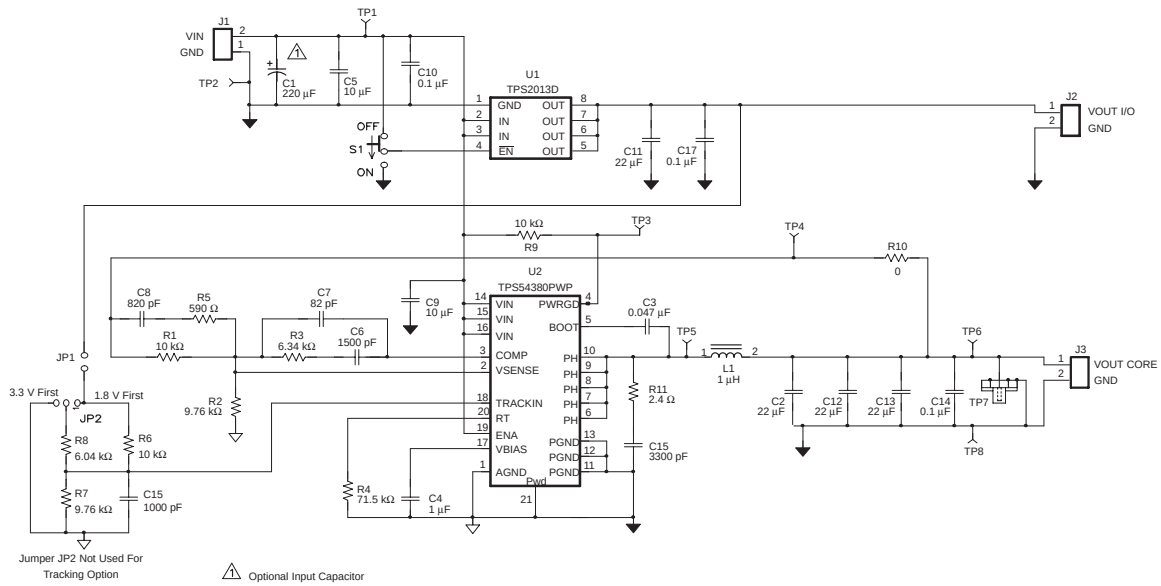
Figure 4-1. TPS54380EVM-001 Schematic
