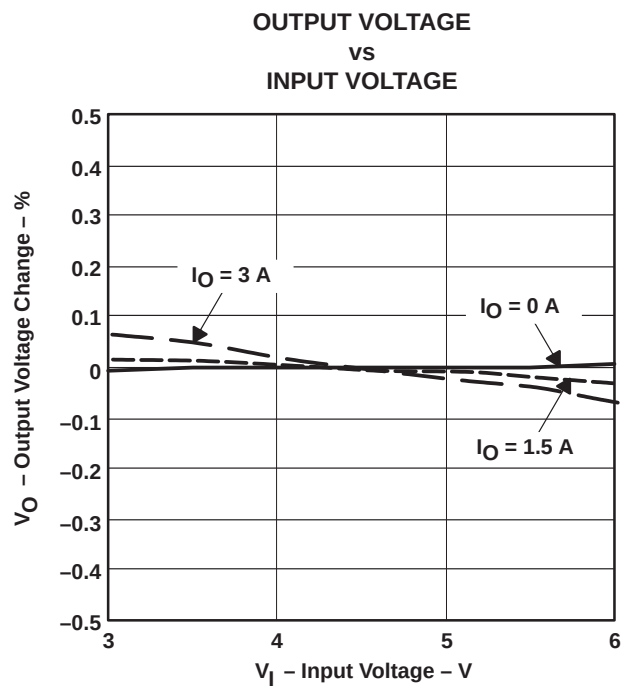
Figure 2-5. Line Regulation
