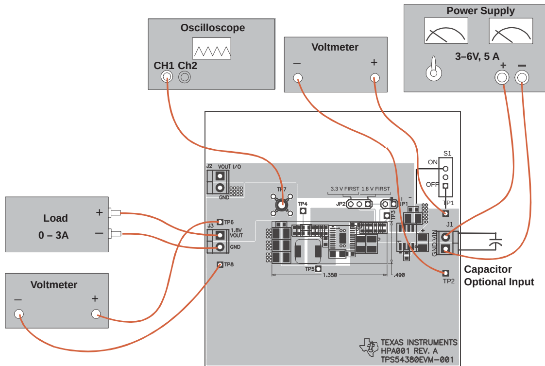
Figure 2–1. Connection Diagram
